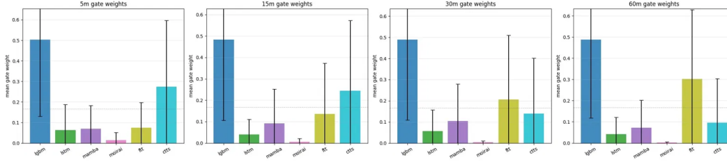
Figure 3: Mean gate weight per expert across the test set, by horizon. Error bars show \pm 1 standard deviation.
